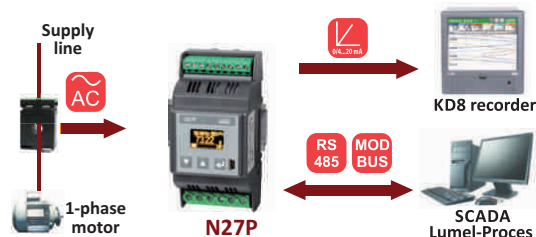
indirect measurement
