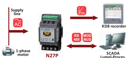
direct measurement
